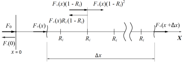
Fig. 1. Outline of the 1D scattering problem without absorption illustrating the structure of the interval \Delta x . The formation of transmitted and backscattered fluxes is shown through the example of the second scatterer at \Delta x .
