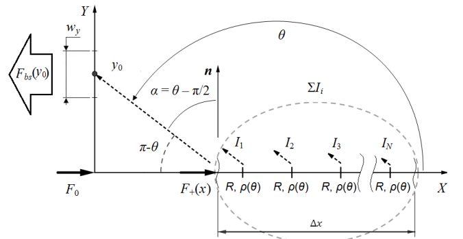
Fig. 2. Outline of the 2D scattering problem without absorption illustrating the structure of the interval \Delta x and formation of the scattered flux.
